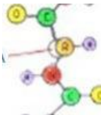
Cheratina
